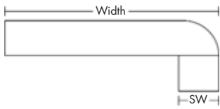
Built Up Edge Single Postform
